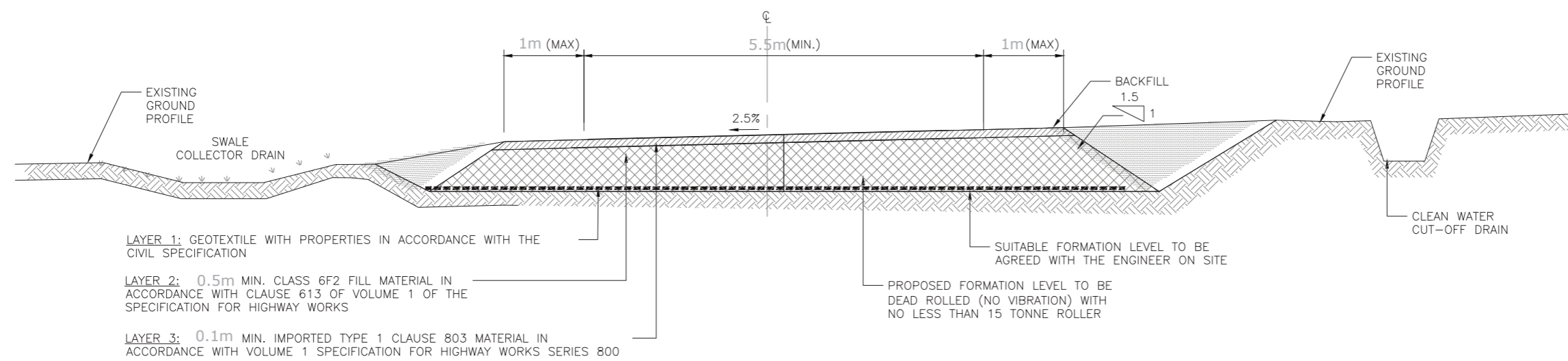
TYPICAL SECTION OF CUT AND FILL ACCESS TRACK
